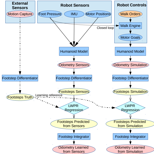
Fig. 4: System architecture. Ellipses represent values and rectangles represent abstract functions. All odometry estimations (red) are compared with ground truth motion capture.
