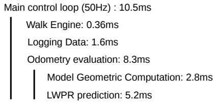
Fig. 6: Average computing time on robot's embedded CPU
