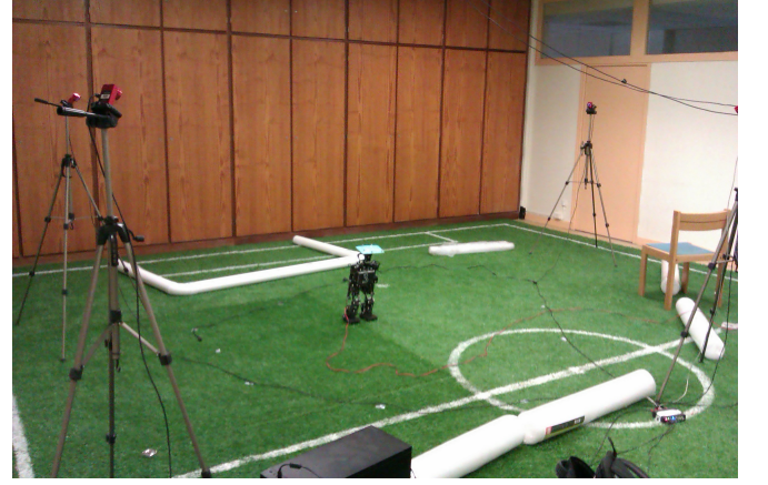
Fig. 5: The motion capture area on artificial grass (30mm thick) field and Sigmaban humanoid robot with reflective markers on the head
