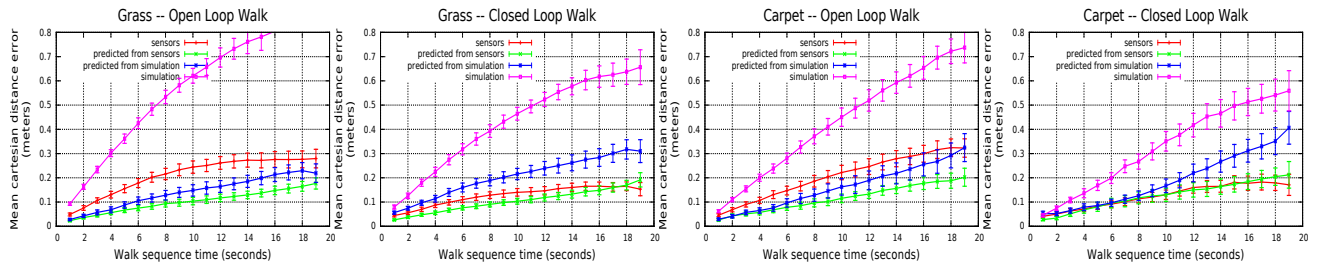
Fig. 10: Comparison of odometry error using closed-loop and open-loop walk engines and artificial grass and carpet surfaces. Each comparison is made of 45 to 72 walk sequences of 20 seconds.
