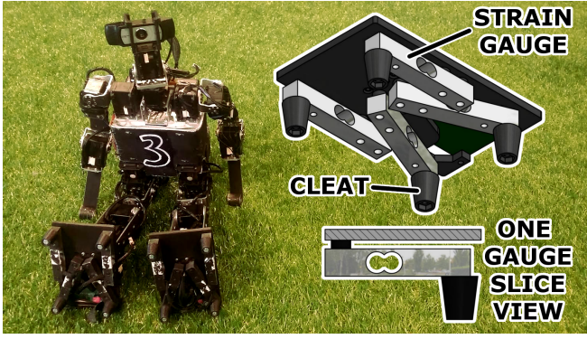
Fig. 1: On the left side, Sigmaban Kid-Size Humanoid Robot. On the right side, low-cost foot pressure sensors made of 4 strain gauges and measuring weight put on each cleat. This mechanical assembly is robust and well adapted to soft artificial grass, improving the stability of the robot
