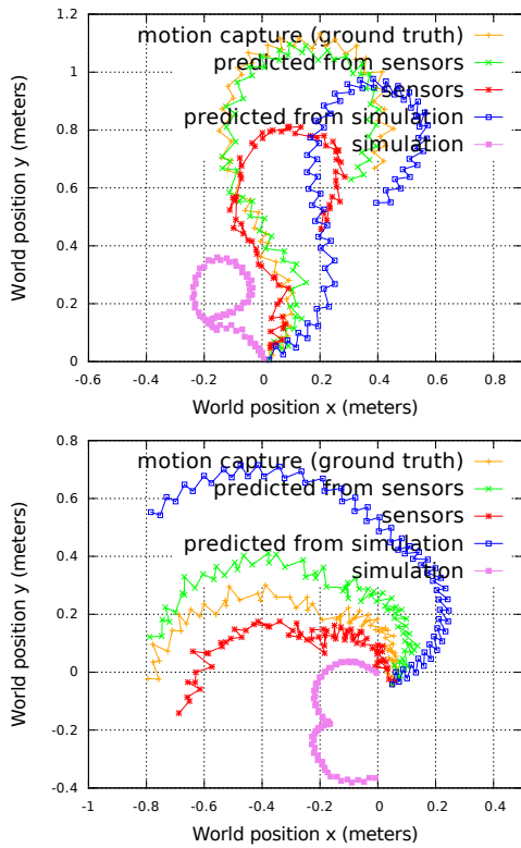
Fig. 8: The four odometry methods compared with motion capture measured ground truth on two typical walk sequences. The integrated robot’s head trajectory is shown over a walk time length of 20 seconds starting from the origin (0,0) position. Forward steps, lateral steps and turn walk inputs are mixed. Due to control errors, a stationary or slightly negative forward order may results in a forward motion. On both trajectory beginnings, actual stationary turn is performed, misleading the simulation-based odometry which integrates backward displacements.
