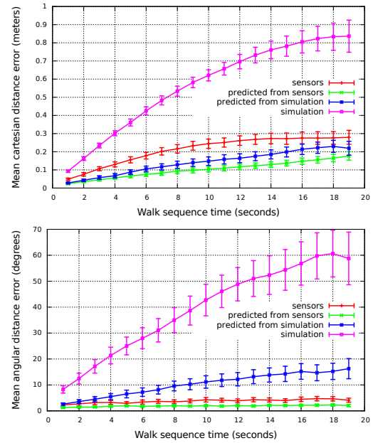
Fig. 9: Average distance of Cartesian and angular odometry from ground truth. Comparison of the four odometry methods statistics from 58 walk sequences of 20 seconds. Error bars give 95% confidence intervals on average.
