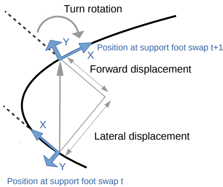
Fig. 3: Footstep displacement calculations on support foot swap
