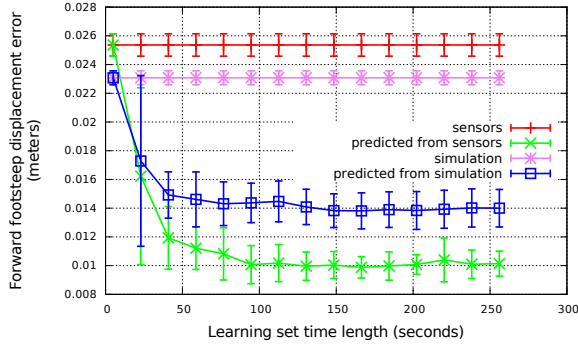
Fig. 7: Average distance between estimated footstep displacement in the robot's forward direction (x) and measured ground truth. Comparison of footstep displacements computed from motors goals (violet) and sensors (red) versus regression predictions (green and blue) under different learning time durations. Error bars give 95% confidence intervals evaluated from 5 logs.
